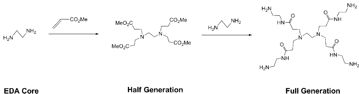
Figure 2. Synthesis of G 0 -NH 2 as an example for the synthesis of PAMAM dendrimers. Ethylene diamine (EDA) core reacts with methyl acrylate monomers via a Michael addition reaction and yields a branched intermediate (half generation) that reacts with excess EDA to produce the complete G 0 -NH 2 dendrimer.
